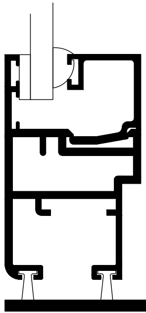
GOAL-POST FRAME WITH 3mm SILL PLATE
