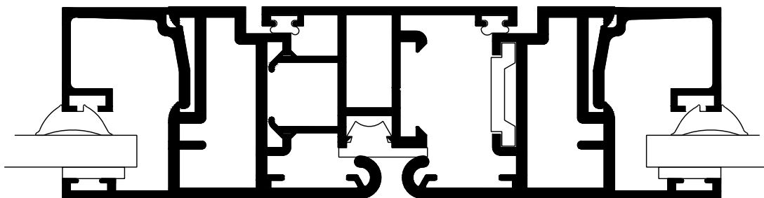
5 DOUBLE CASEMENT MEETING STILE
