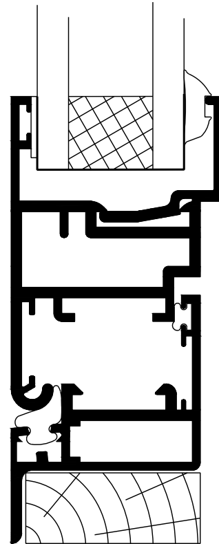
28mm DOUBLE GLAZED UNIT
